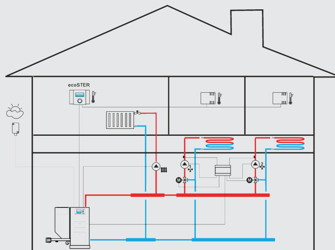
Figure 2- ecoSTER 200 with 3 room sensors
