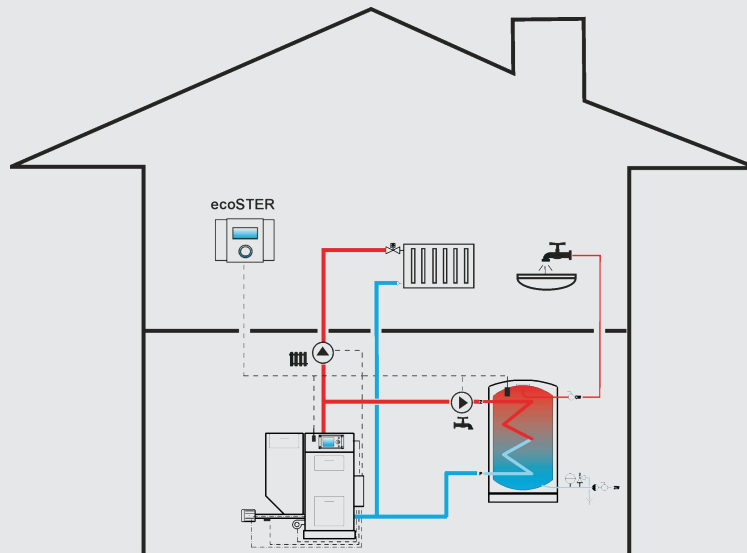
Figure 1- ecoSTER 200 (internal room sensor)
